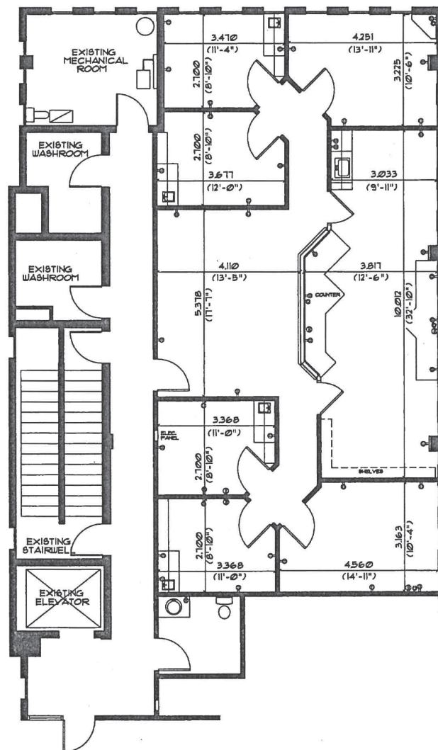
FIFTH FLOOR PLAN
